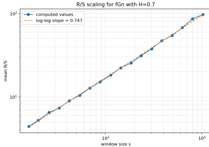
Figure 4: R/S scaling plot for fGn with H = 0.7 .
