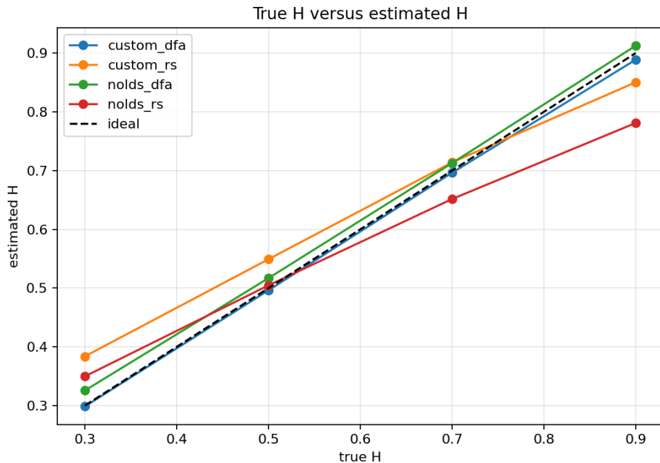
Figure 6: True H versus estimated H .
