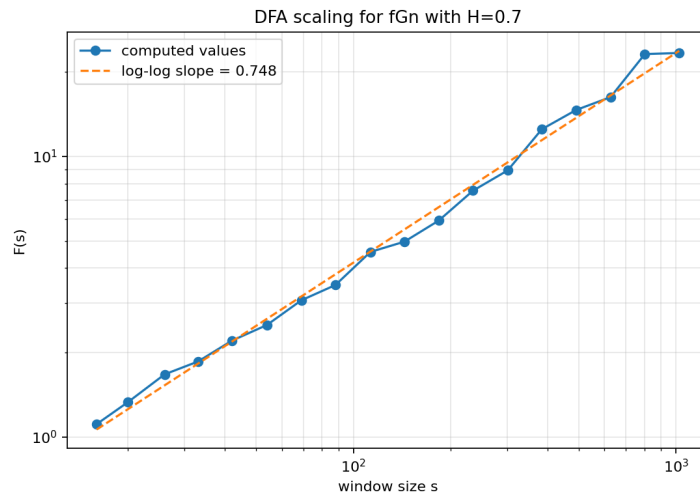
Figure 5: DFA scaling plot for fGn with H = 0.7 .
